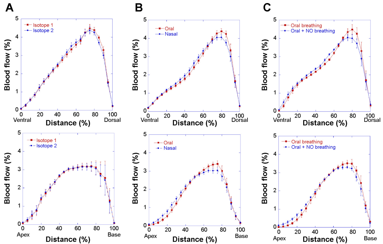
Fig. 2. Relative distribution of pulmonary blood flow along the distance from the apex to base regions and from the ventral to dorsal regions under the simultaneous administration of both radiotracers (A), a switch from oral to nasal breathing (B), and a switch from oral breathing of NO-free air to oral breathing of air enriched with exogenous NO (C). Values are means \pm SD.
