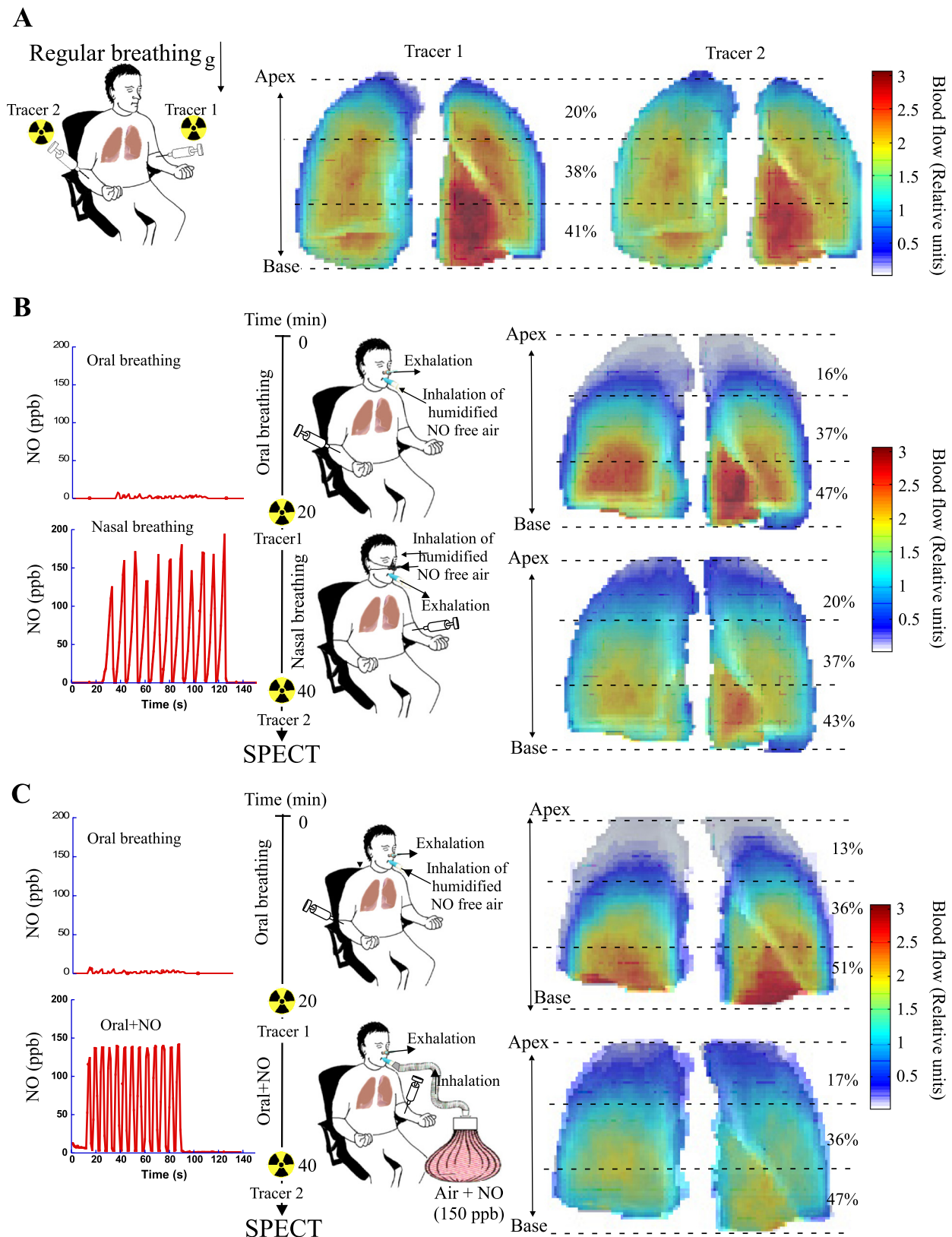
Fig. 1. A , left: the two different tracers ( tracers 1 and 2 ) were simultaneously administered in subjects in group A . The single-photon emission computed tomography (SPECT) results are presented for one of the subject in group A in the middle and right images, respectively, for tracers 1 and 2 . The dashed lines mark the three lung compartments in the cranial-caudal direction and the values the relative perfusion distribution within each compartment. B , left: levels of endogenous nitric oxide (NO) measured in the oropharynx of a volunteer during oral and nasal breathing. Middle , timeline for the different breathing patterns. The different tracers were injected at the indicated time points. Right , SPECT results for each breathing pattern. C : effects of oral inhalation with the addition of exogenous NO on lung perfusion in one subject in group C . ppb, parts per billion.
