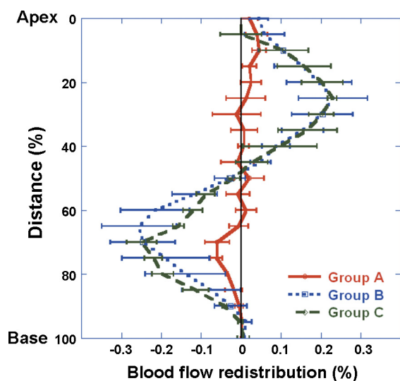
Fig. 3. Curves representing the blood flow distribution during NO inhalation (endogenous for group B or exogenous for group C ) minus the blood flow distribution during oral breathing NO free air. For group A , the curve represents the difference in blood flow distributions as mapped with the two radiotracers simultaneously administered under regular breathing conditions.
