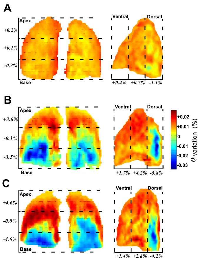
Fig. 4. A: frontolateral lung images showing the differences in blood flow distribution as mapped with two distinct tracers simultaneously administered under regular breathing conditions. B and C: frontolateral lung images showing the regional variations in blood flow distribution resulted when changing from oral breathing (first tracer) to nasal breathing (second tracer) or from oral breathing NO free air to oral breathing exogenous NO, respectively. The dashed lines limit the nine volumes of interest, each representing one-third of the lung distance from apex to base regions and from the ventral to dorsal regions.
